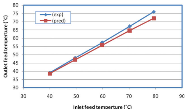
Figure 14. Relationship between the outlet and inlet temperature of the feed stream. 48
