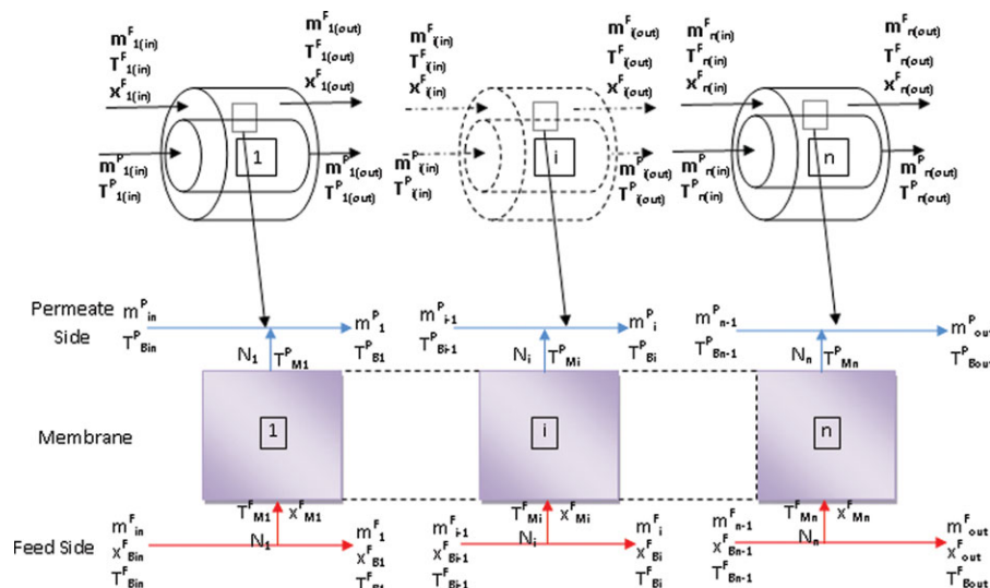
Figure 3. Schematic representations of the DCMD general concept cells.
