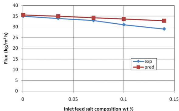
Figure 10. Effect of salt concentration on permeate flux of PP membrane. 46
